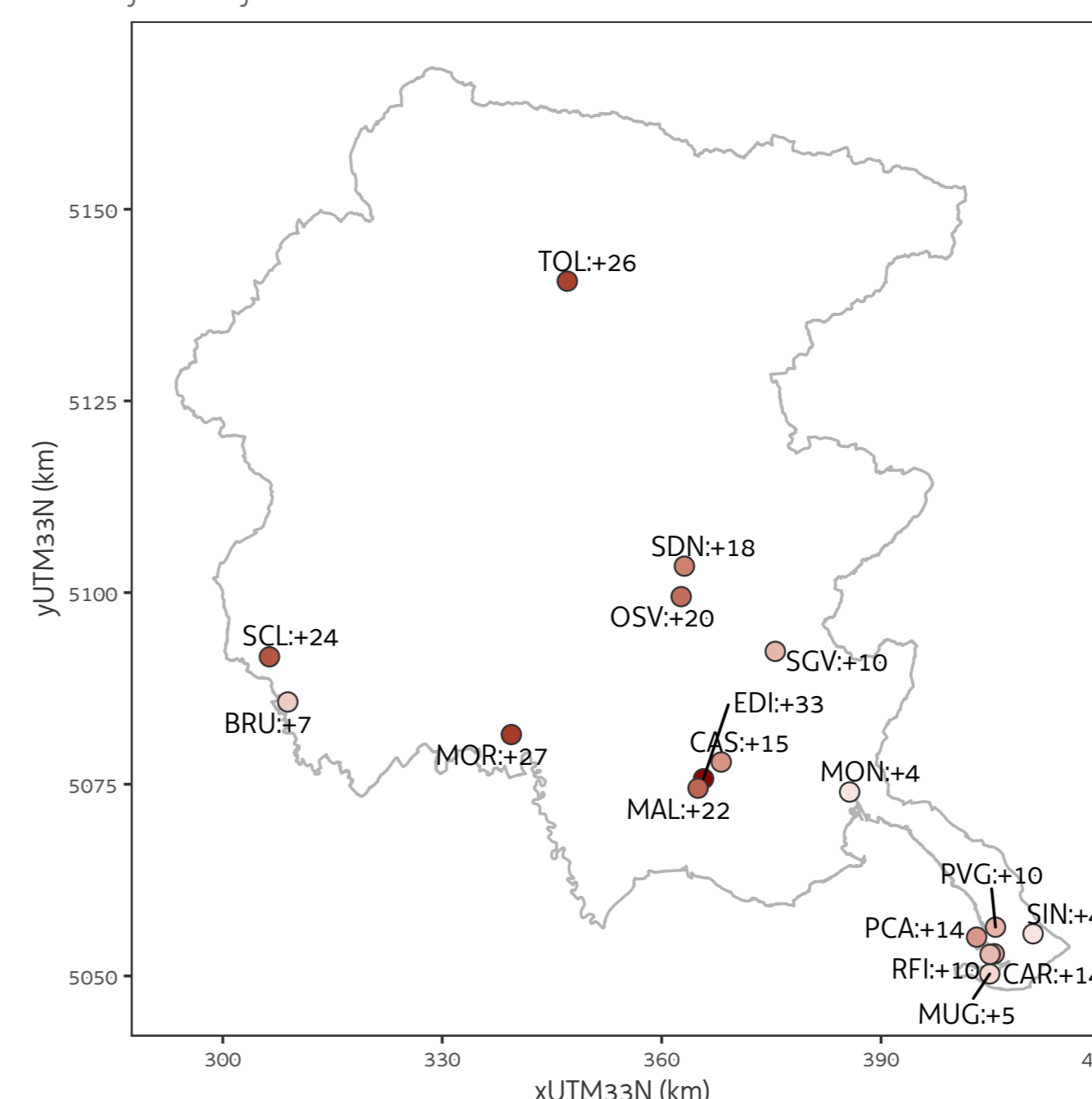
differences in PM2.5 maxima forecast: from 2019-02-09 to 2019-02-13
