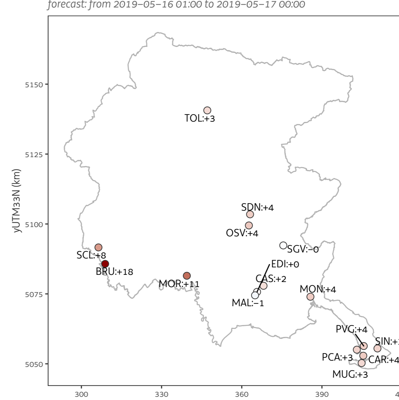
differences in PM10 maxima (bc_Chimere-bc_Farm) forecast: from 2019-05-16 01:00 to 2019-05-17 00:00
